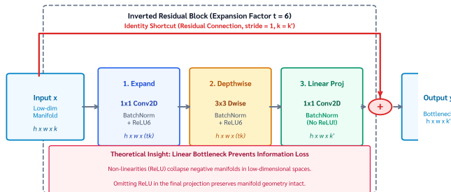
Panel (b): MobileNetV2 Inverted Residual Block with Linear Bottleneck
